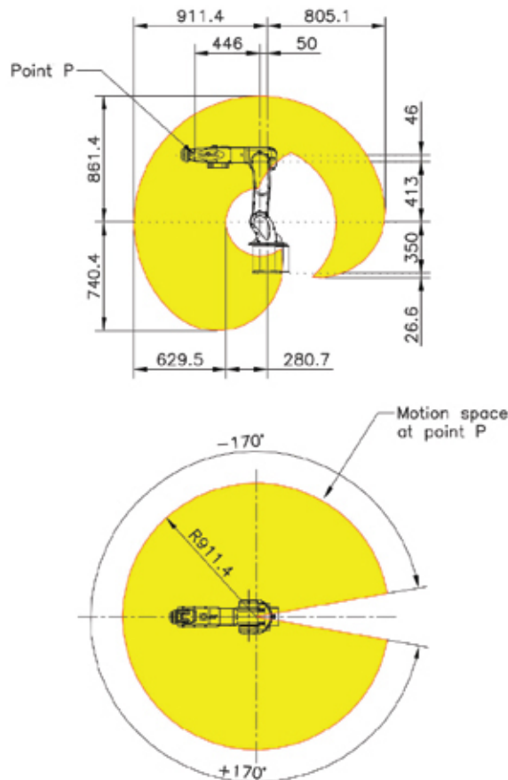
iR18-800
