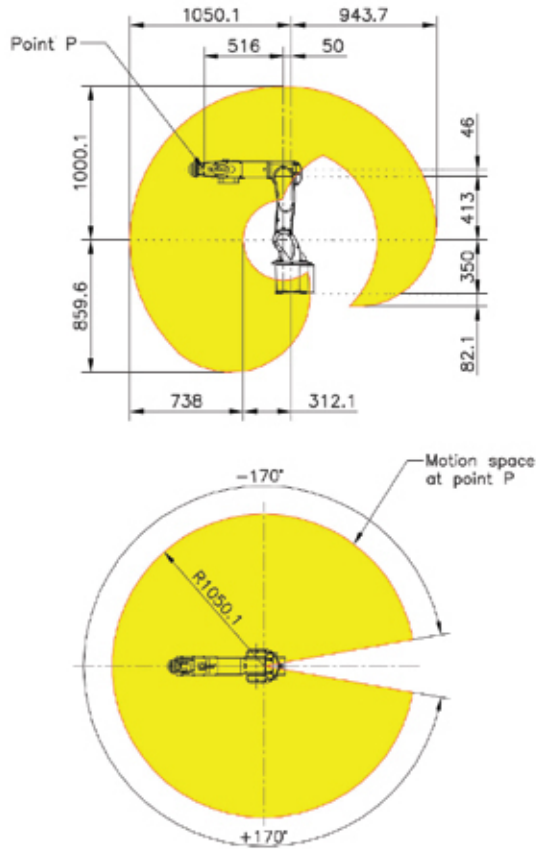
iR18-1000
