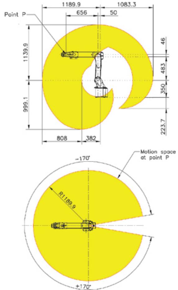
iR18-1200
