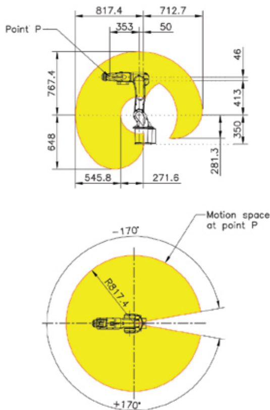
iR18-600
